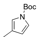
tert -butyl 3-methyl-1H-pyrrole-1-carboxylate ( 3 ) 1 H NMR (400MHz, CDCl 3 )
